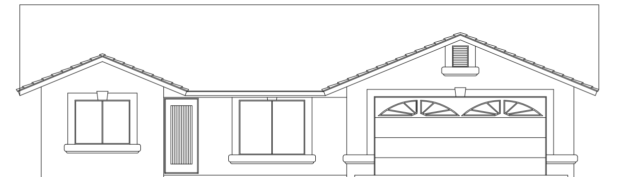
FRONT ELEVATION
