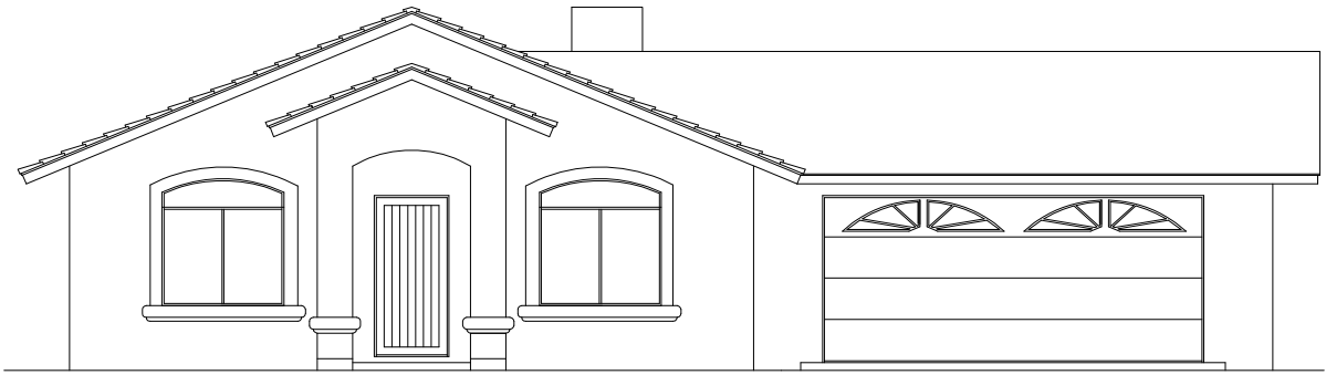
FRONT ELEVATION W/ OPTIONS
