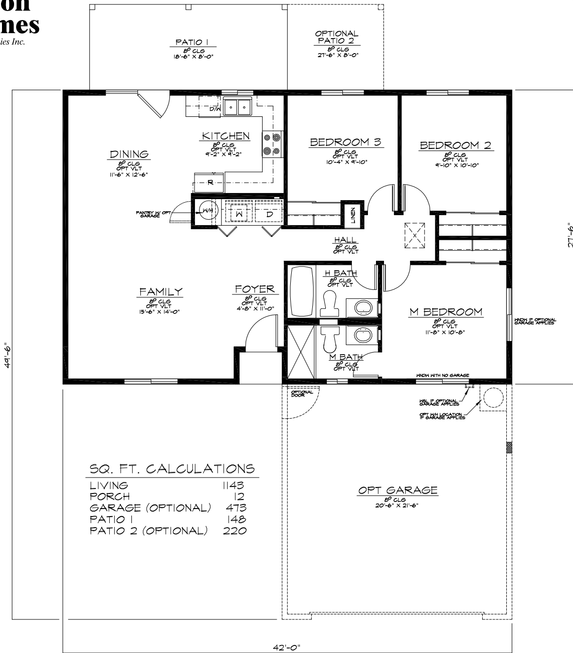
FLOOR PLAN
