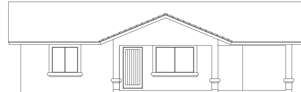
FRONT ELEVATION W/ OPT PORCH
