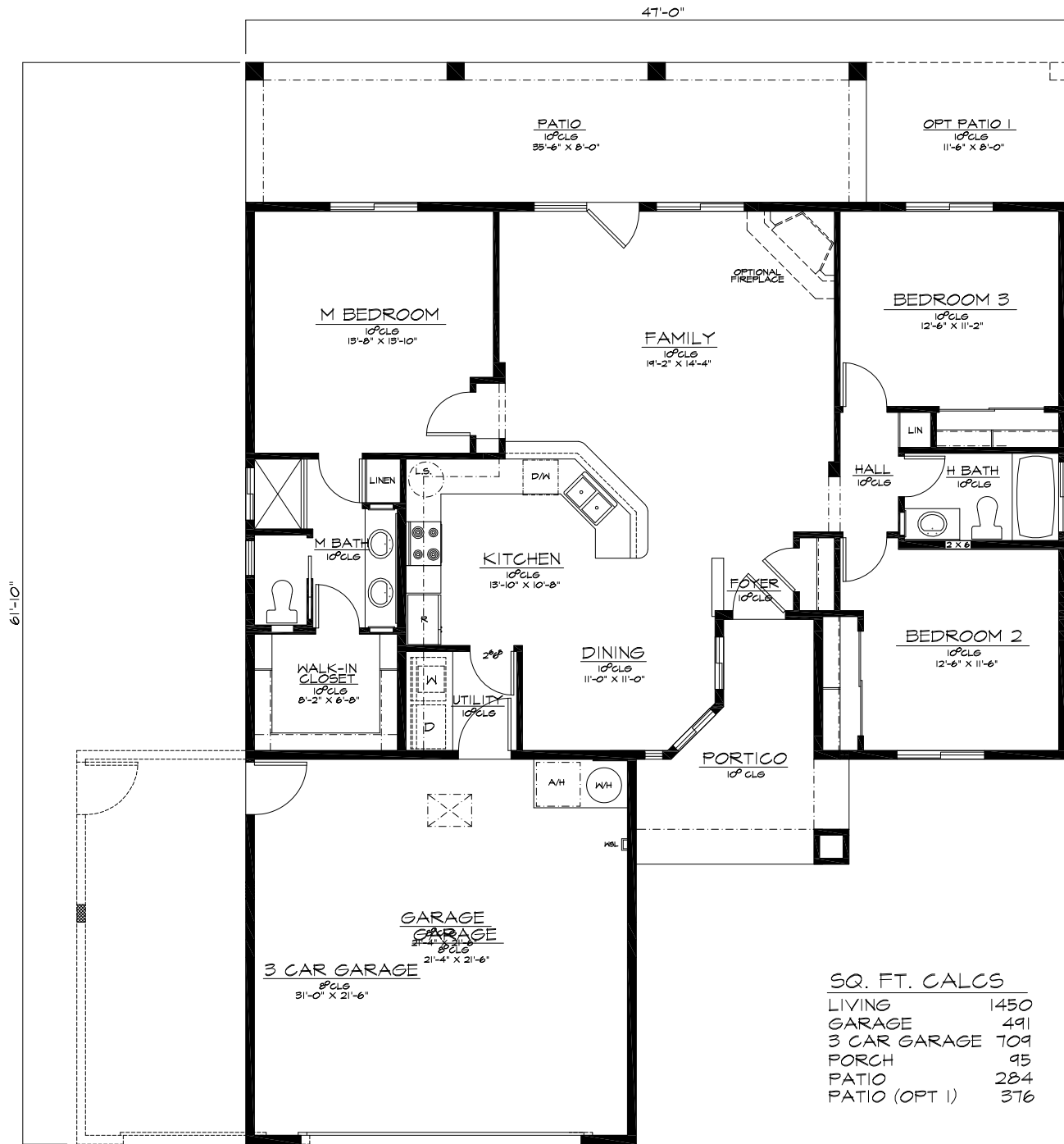
FLOOR PLAN
