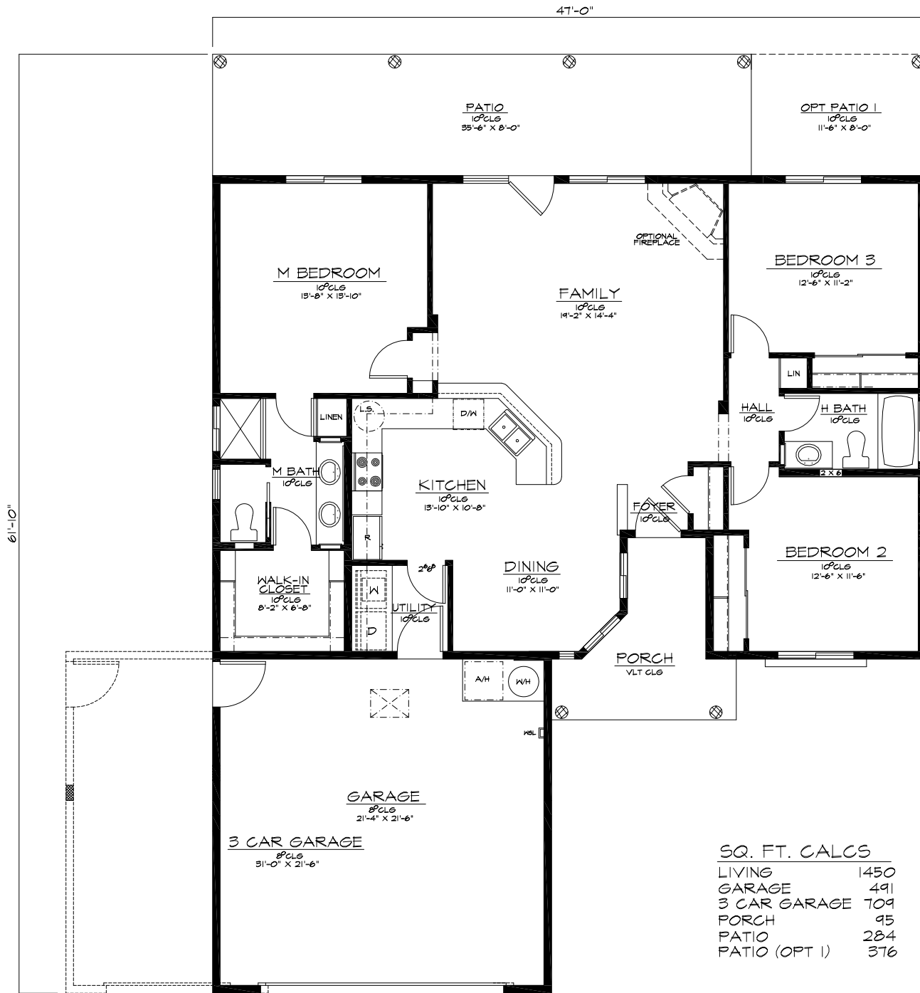
FLOOR PLAN
