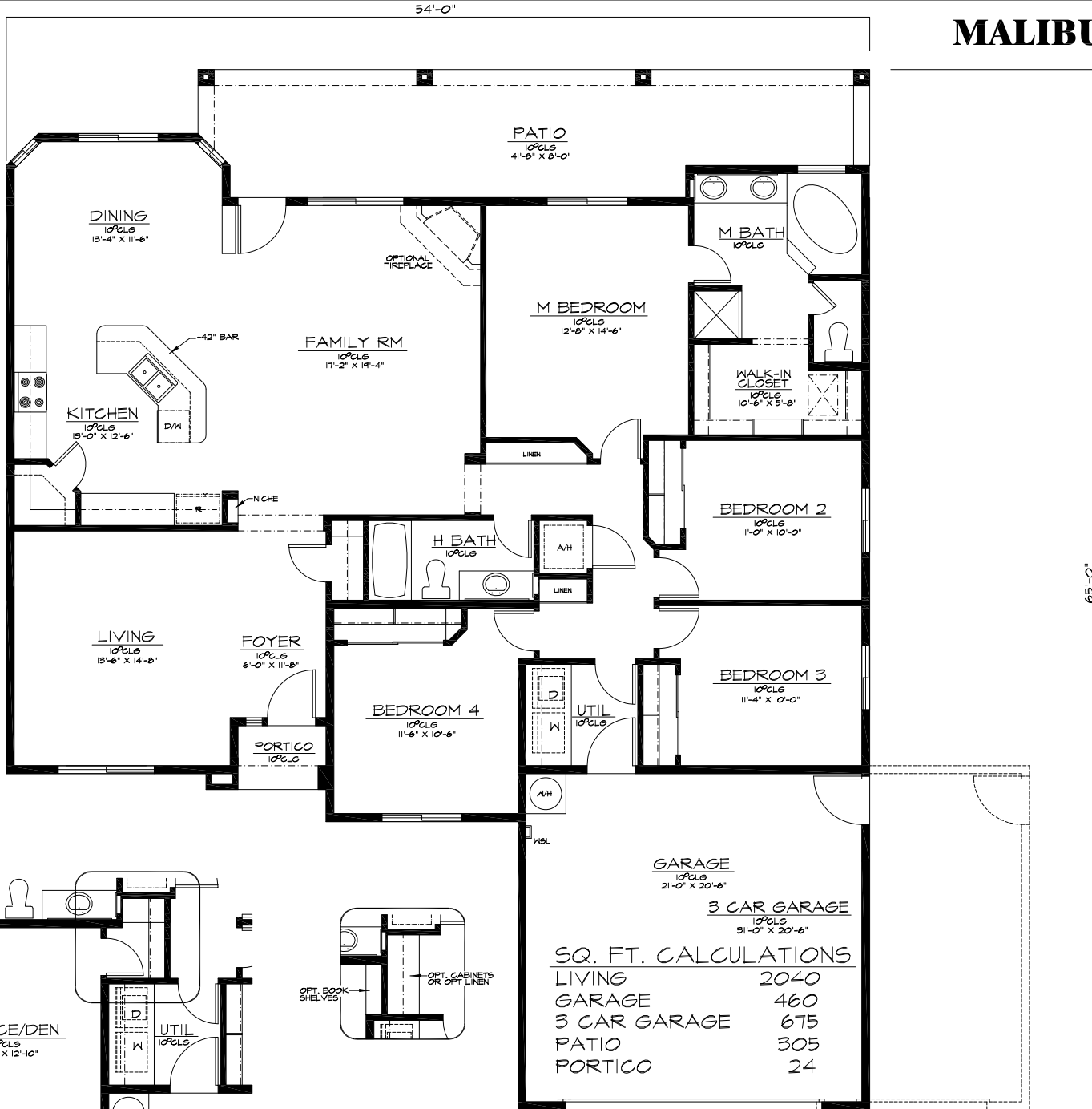
FLOOR PLAN
