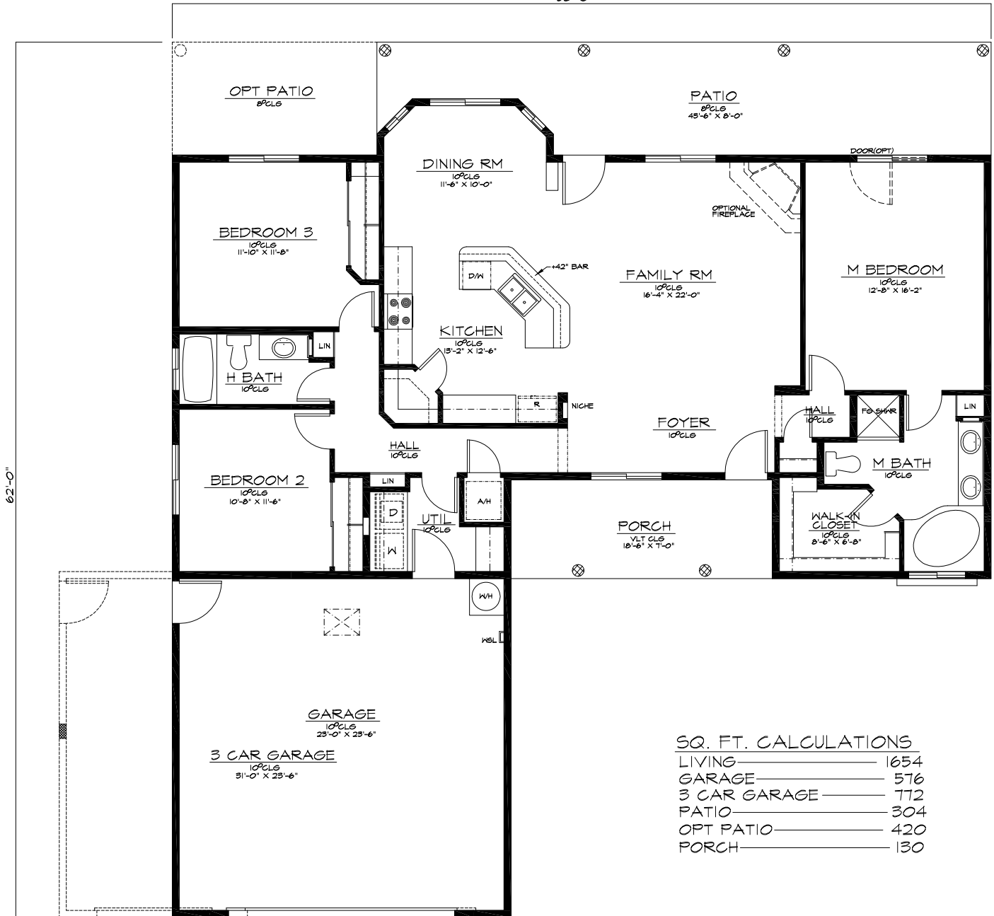
FLOOR PLAN
