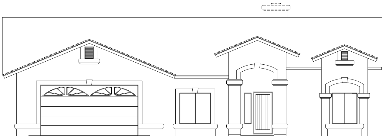
FRONT ELEVATION
