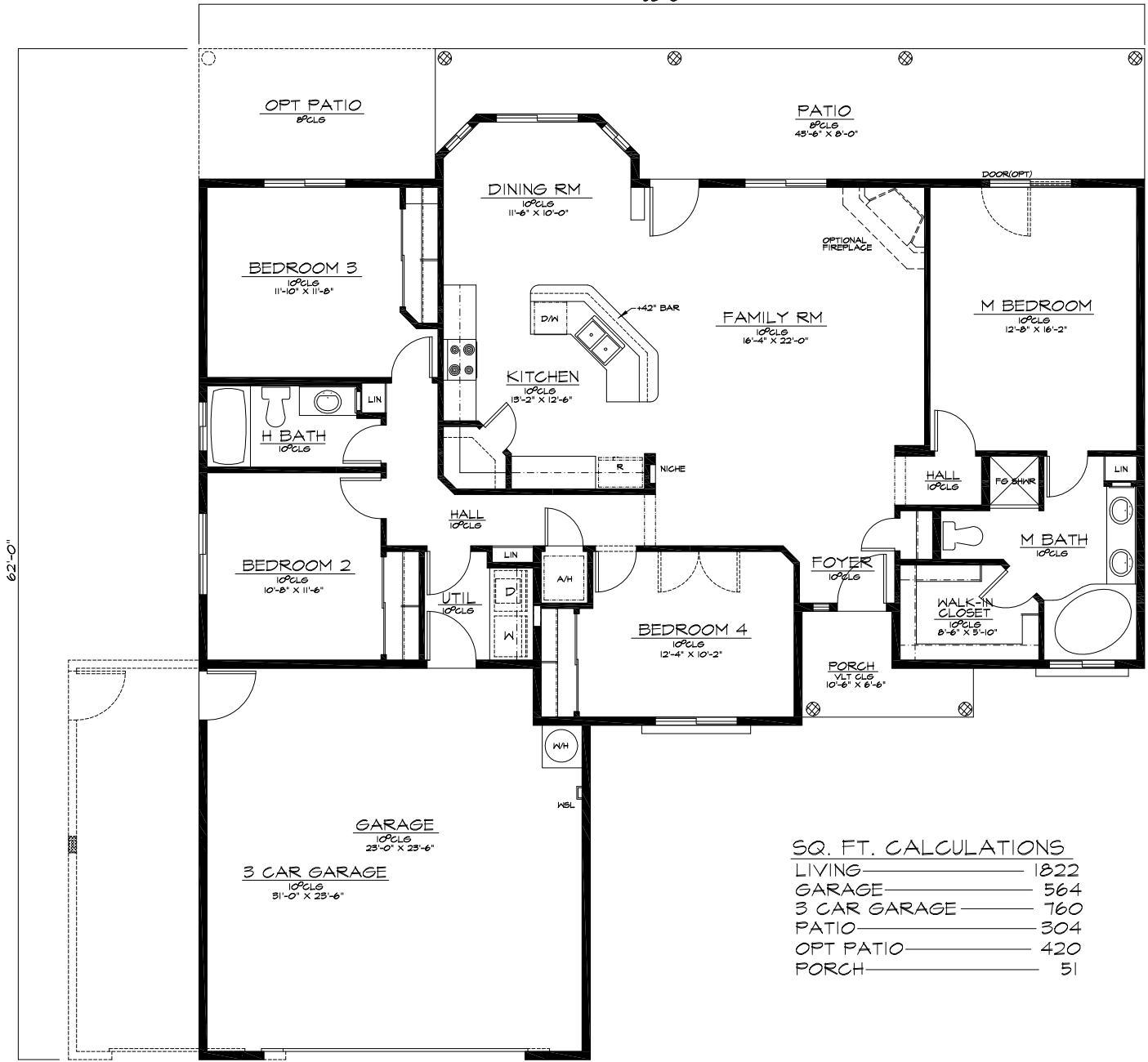
FLOOR PLAN
